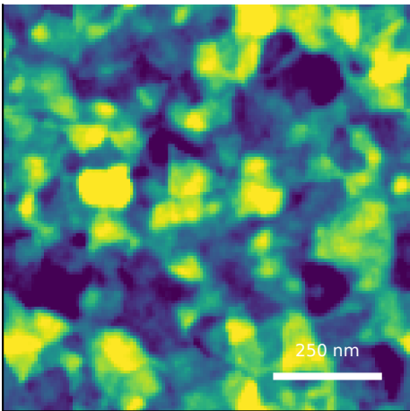
generated AFM predicted Sq=3.56 nm; FSMI=3.15 nm C=29/100
