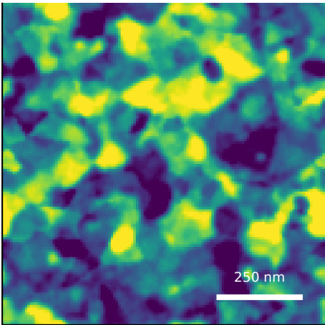
generated AFM predicted Sq=1.94 nm; FSMI=1.74 nm C=66/100
