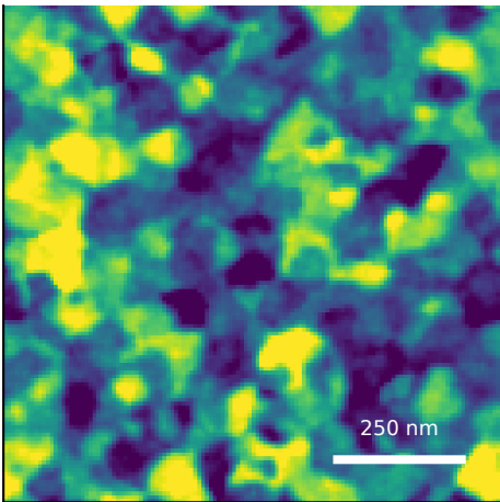
generated AFM predicted Sq=1.35 nm; FSMI=1.19 nm C=83/100
