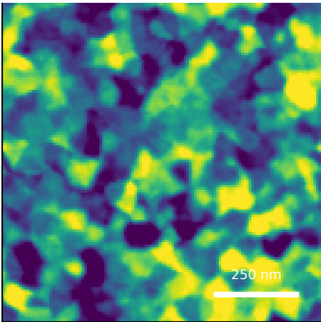
generated AFM predicted Sq=1.74 nm; FSMI=1.53 nm C=74/100
