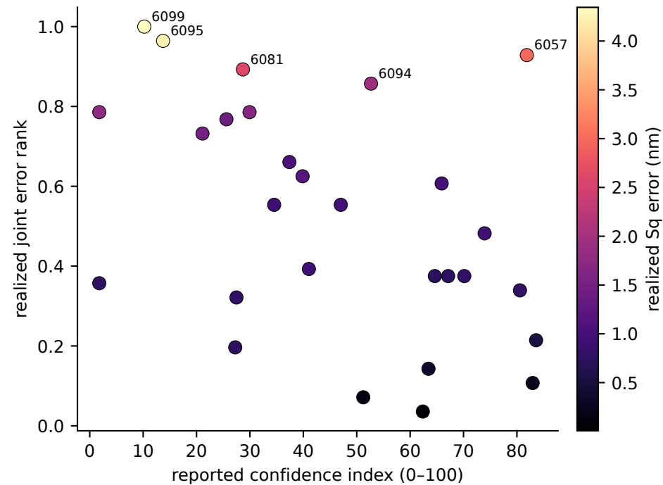
Confidence is error-related: Spearman \rho=-0.42 , p=0.026
