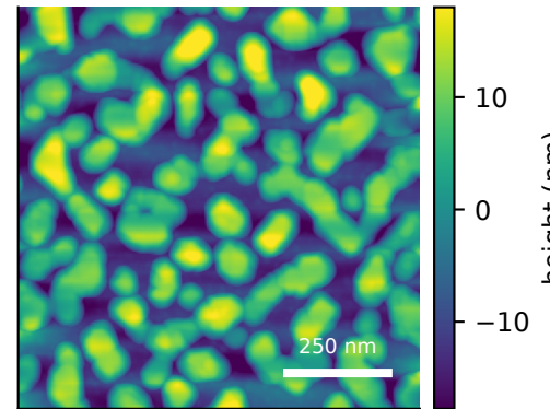
measured AFM displayed scan S_q=9.39 nm sample median S_q=9.39 \pm 0.21 nm (IQR)
