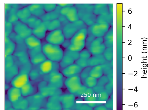
measured AFM displayed scan S_q=2.00 nm sample median S_q=3.35 \pm 3.02 nm (IQR)
