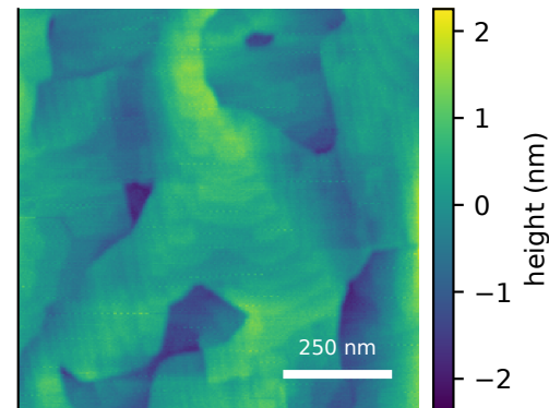
measured AFM displayed scan S_q=1.56 nm sample median S_q=1.50 \pm 0.18 nm (IQR)
