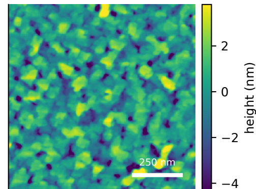
measured AFM displayed scan S_q=2.18 nm sample median S_q=2.24 \pm 0.18 nm (IQR)
