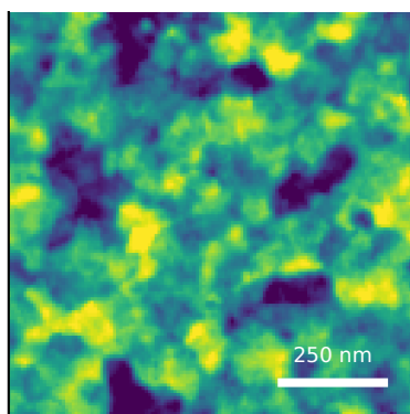
M10 baseline predicted S_q=2.40 nm
