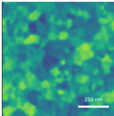
generated AFM predicted Sq=0.97 nm; FSMI=0.86 nm C=82/100
