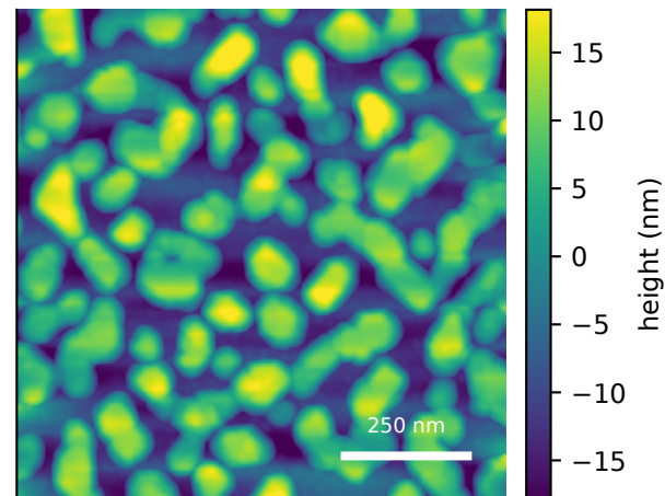
measured AFM displayed scan Sq=9.07 nm sample median Sq=9.07 ± 2.19 nm (IQR)
