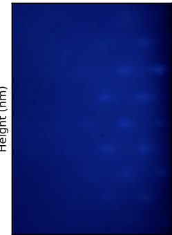
Sample 6029 RHEED Manual selection select_after_ramping_down_GaSb.jpg
