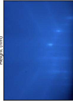
Sample 6073 RHEED Manual selection select_oxy.jpg
