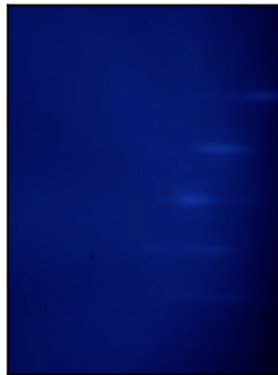
Sample 6101 RHEED Manual selection select_150_min_GaSb.jpg
