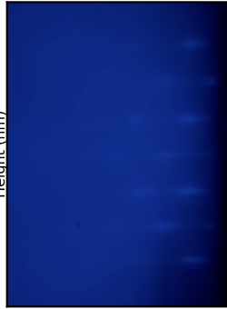
Sample 6072 RHEED Manual selection select_rampdown_to_250C.jpg
