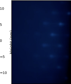
Sample 6063 RHEED Manual selection select_rampdown_to_300C.jpg
