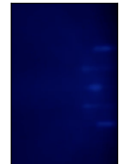
Sample 6023 RHEED Manual selection select_after_ramping_down.jpg
