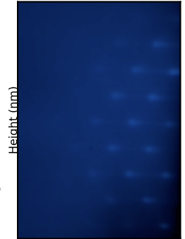
Sample 6080 RHEED Manual selection select_after_rampdown_to_200C.jpg
