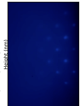
Sample 6099 RHEED Manual selection select_ramping_to_650C.jpg
