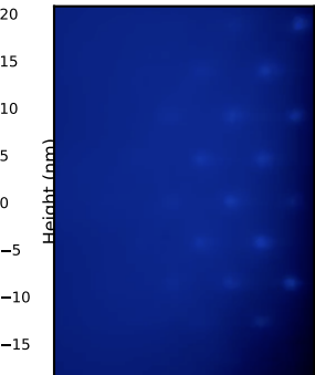
Sample 6095 RHEED Manual selection select_rampdown_to_250C.jpg
