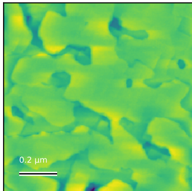
N6022_Ctr_004 Rq=1.4 nm; 1 x 1 \mu\text{m}
