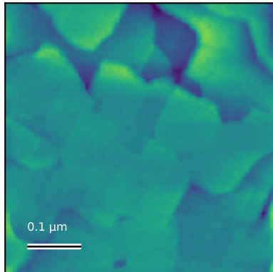
N6022_Ctr_001 Rq=0.81 nm; 0.5 x 0.5 \mu\text{m}
