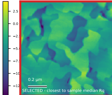
N6022_Ctr_000 Rq=1.6 nm; 1 x 1 \mu\text{m}
