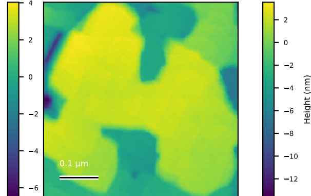
N6022_Ctr_003 Rq=2.6 nm; 0.5 x 0.5 \mu\text{m}
