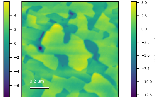
N6022_Ctr_002 Rq=1.9 nm; 1 x 1 \mu\text{m}
