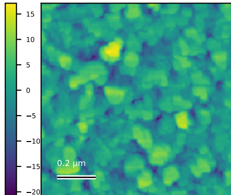
N6028_500_nm_006 Rq=2.3 nm; 1 x 1 \mu m
