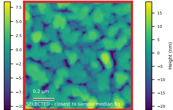
N6028_1um_004 Rq=6.1 nm; 1 x 1 \mu m
