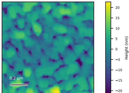
N6028_1um_003 Rq=6.2 nm; 1 x 1 \mu m
