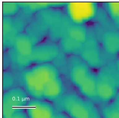
N6028_500_nm_005 Rq=5.8 nm; 0.5 x 0.5 \mu m
