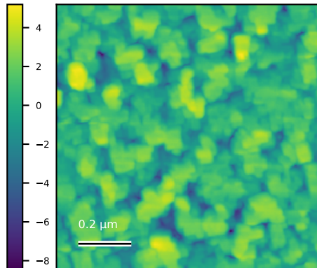
N6029_1um_007 Rq=2.3 nm; 1 x 1 \mu\text{m}
