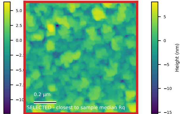
N6029_1um_008 Rq=2.6 nm; 1 x 1 \mu\text{m}
