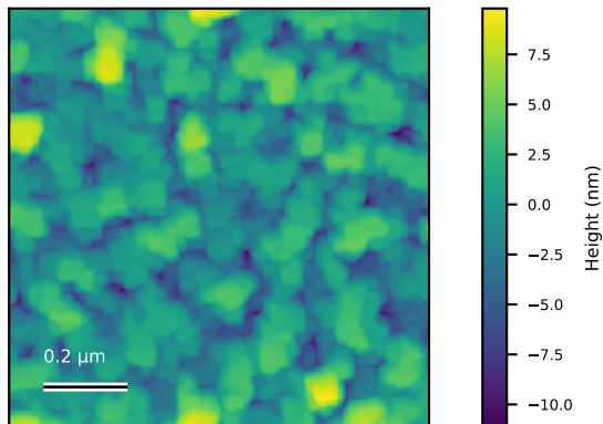
N6029_500_nm_010 Rq=3 nm; 1 x 1 \mu\text{m}
