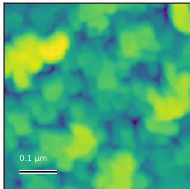
N6029_500_nm_009 Rq=2.1 nm; 0.5 x 0.5 \mu\text{m}
