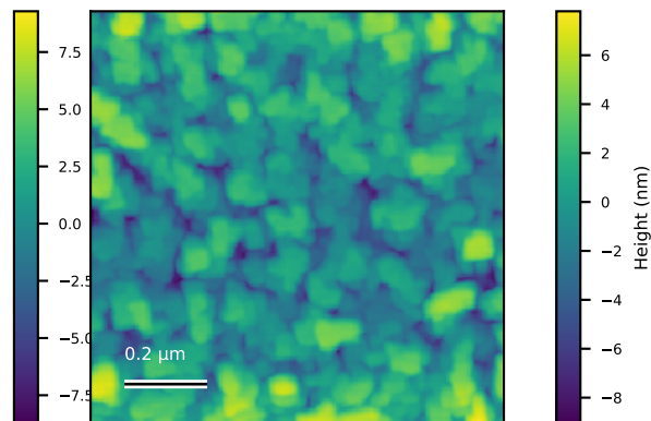
N6033_1um_018 Rq=2.5 nm; 1 x 1 \mu m
