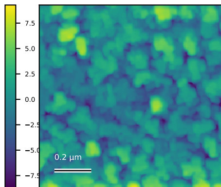
N6033_1um_017 Rq=2.5 nm; 1 x 1 \mu m
