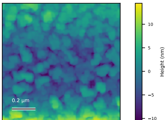
N6033_1um_015 Rq=3.8 nm; 1 x 1 \mu m
