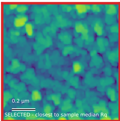
N6033_1um_016 Rq=2.5 nm; 1 x 1 \mu m
