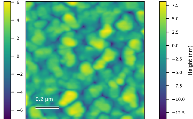
N6041_1um_000 Rq=3.2 nm; 1 x 1 \mu\text{m}
