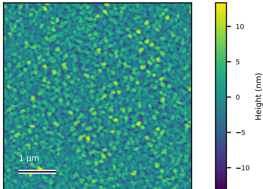
N6041_5um_001 Rq=3.5 nm; 5 x 5 \mu\text{m}
