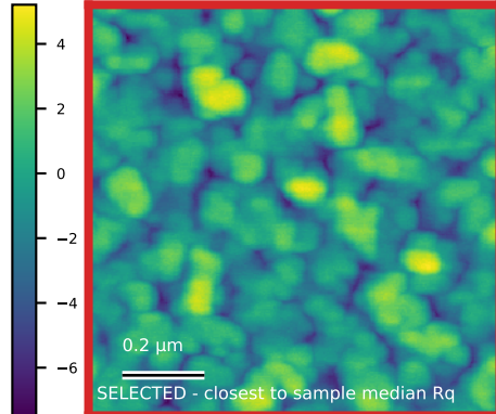
N6041_1um_003 Rq=2 nm; 1 x 1 \mu\text{m}
