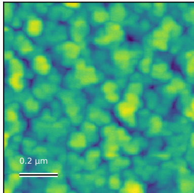
N6041_1um_002 Rq=1.9 nm; 1 x 1 \mu\text{m}
