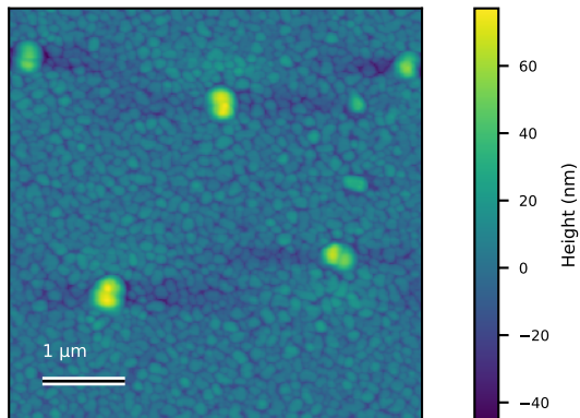
N6043_5um_002 Rq=10 nm; 5 x 5 \mu\text{m}
