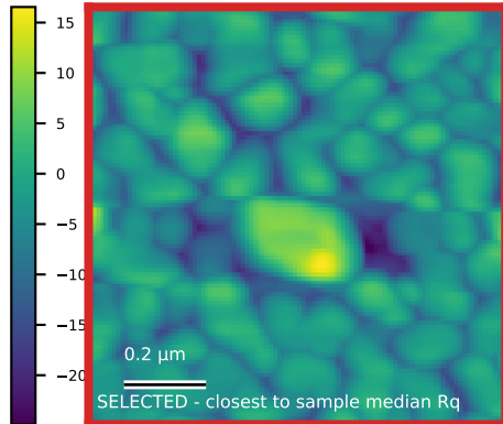
N6043_1um_3 Rq=7.4 nm; 1.016 x 1.016 \mu\text{m}
