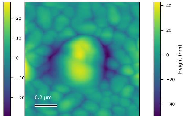
N6043_1um_2 Rq=13 nm; 1.016 x 1.016 \mu\text{m}
