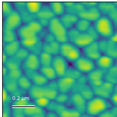
N6043_1um_cs Rq=6 nm; 1.016 x 1.016 \mu\text{m}
