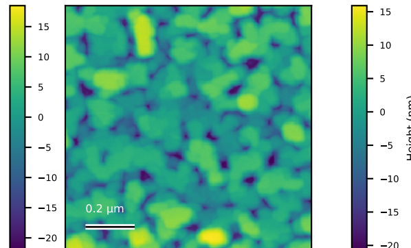
N6047_1um_006 Rq=5.6 nm; 1 x 1 \mu\text{m}
