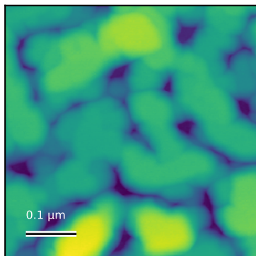
N6047_0.5um_005 Rq=7 nm; 0.5 x 0.5 \mu\text{m}
