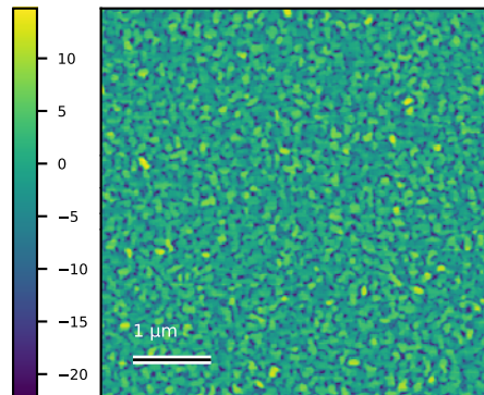
N6047_5um_009 Rq=5.3 nm; 5 x 5 \mu\text{m}
