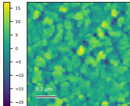
N6047_1um_012 Rq=1.9 nm; 1 x 1 \mu\text{m}
