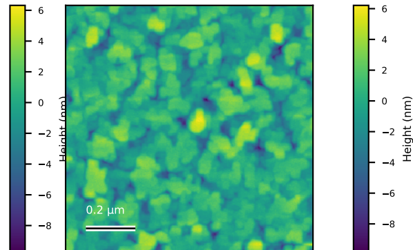
N6047_1um_011 Rq=1.9 nm; 1 x 1 \mu\text{m}
