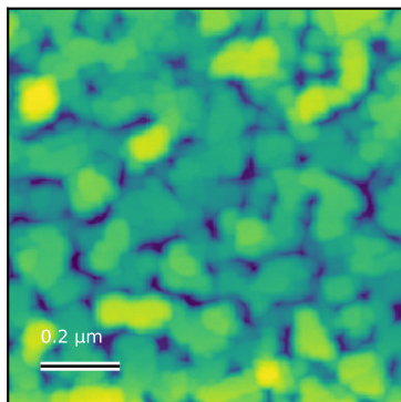
N6047_1um_007 Rq=6.2 nm; 1 x 1 \mu\text{m}
