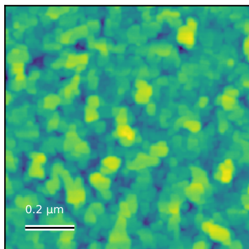
N6047_1um_013 Rq=2 nm; 1 x 1 \mu\text{m}
