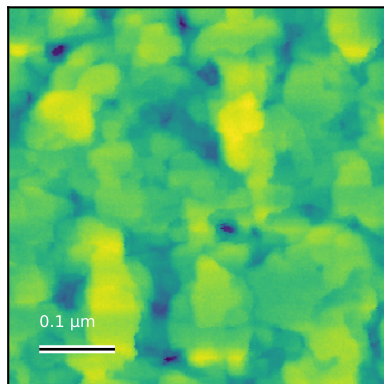
GdSb_N6054_ctr_001 Rq=2.4 nm; 0.5 x 0.5 \mu m
