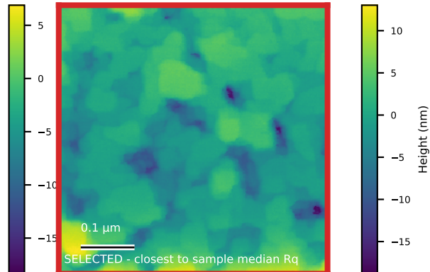
GdSb_N6054_edg_000 Rq=3.7 nm; 0.5 x 0.5 \mu m
