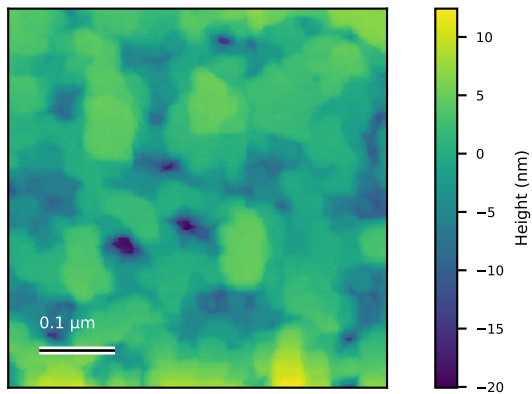
GdSb_N6054_ctr_000 Rq=3.9 nm; 0.5 x 0.5 \mu m
