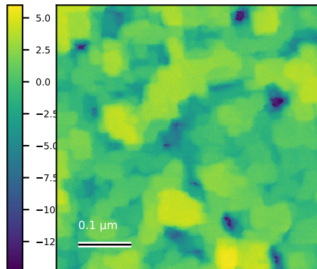
GdSb_N6054_edg_001 Rq=2.8 nm; 0.5 x 0.5 \mu m
