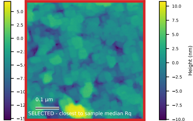
GdSb_N6055_ctr_001 Rq=2.7 nm; 0.5 x 0.5 \mu m
