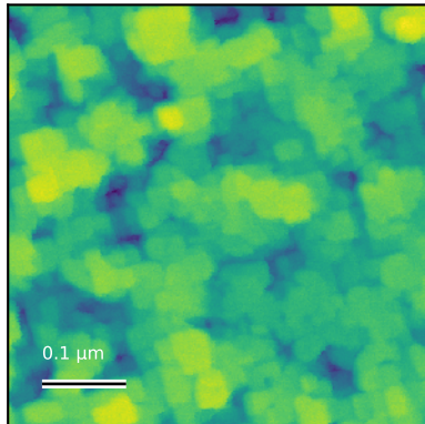
GdSb_N6055_ctr_002 Rq=2.5 nm; 0.5 x 0.5 \mu m
