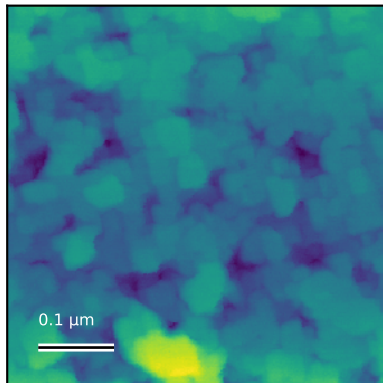
GdSb_N6055_ctr_000 Rq=3.3 nm; 0.5 x 0.5 \mu m
