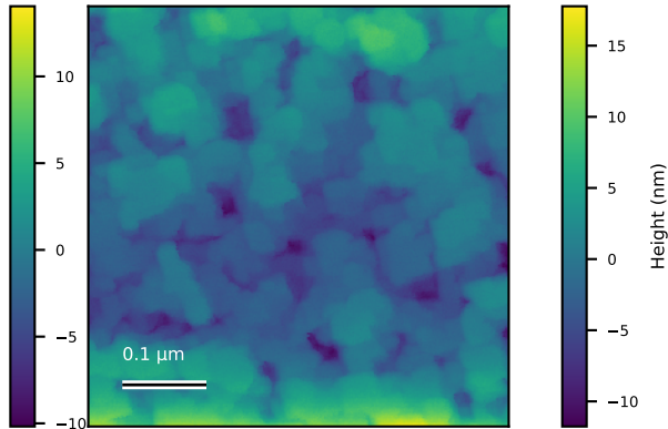
GdSb_N6055_edg_000 Rq=4.1 nm; 0.5 x 0.5 \mu m
