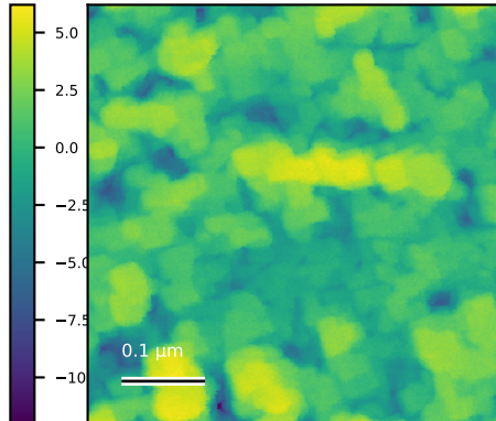
GdSb_N6055_edg_001 Rq=2.6 nm; 0.5 x 0.5 \mu m
