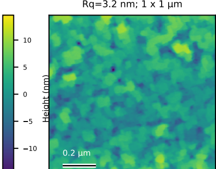
GdSb_N6056_ctr_009 Rq=3.2 nm; 1 x 1 \mu m
