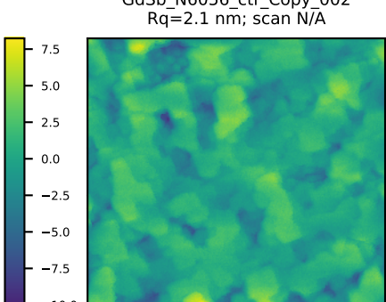
GdSb_N6056_ctr_Copy_002 Rq=2.1 nm; scan N/A
