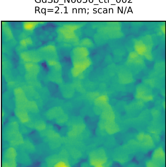
GdSb_N6056_ctr_002 Rq=2.1 nm; scan N/A
