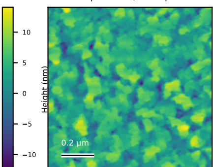
N56_Ctr_002 Rq=2.4 nm; 1 x 1 \mu m
