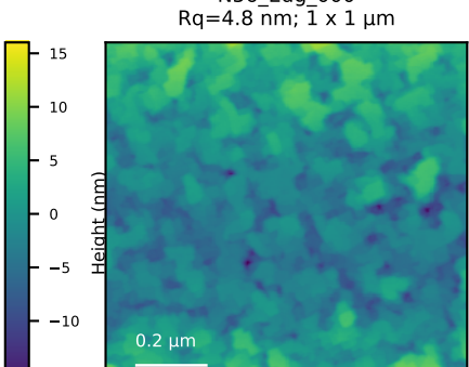
N56_Edg_000 Rq=4.8 nm; 1 x 1 \mu m
