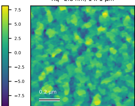
N56_Ctr_003 Rq=2.8 nm; 1 x 1 \mu m
