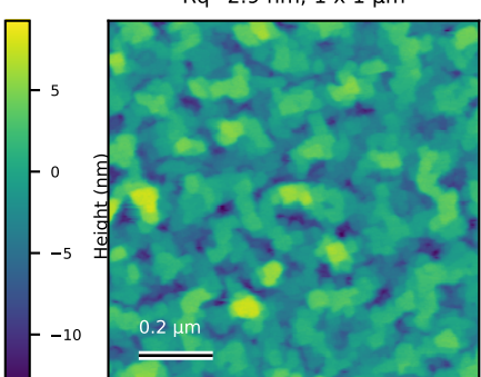
GdSb_N6056_ctr_013 Rq=2.9 nm; 1 x 1 \mu m
