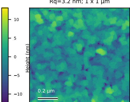
GdSb_N6056_ctr_Copy_005 Rq=3.2 nm; 1 x 1 \mu m
