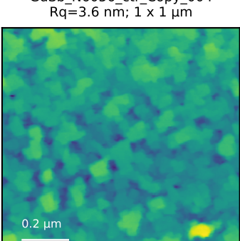
GdSb_N6056_ctr_Copy_004 Rq=3.6 nm; 1 x 1 \mu m
