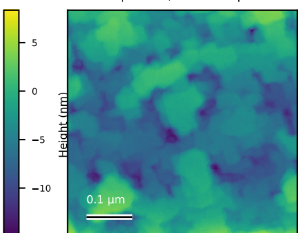
GdSb_N6056_ctr_000 Rq=4 nm; 0.5 x 0.5 \mu m
