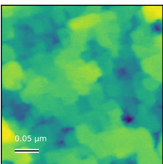
GdSb_N6056_edge_007 Rq=2.1 nm; 0.332031 x 0.332031 \mu m
