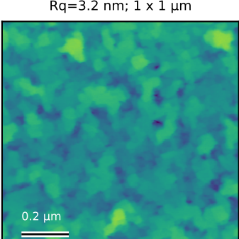
GdSb_N6056_ctr_Copy_006 Rq=3.2 nm; 1 x 1 \mu m
