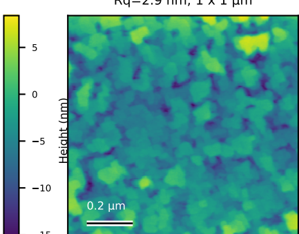
GdSb_N6056_ctr_012 Rq=2.9 nm; 1 x 1 \mu m
