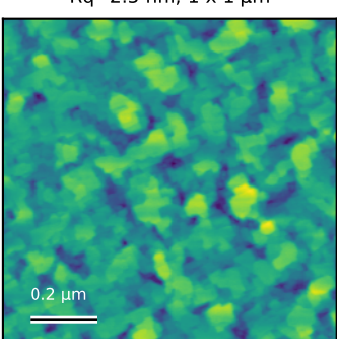
N56_Ctr_001 Rq=2.5 nm; 1 x 1 \mu m
