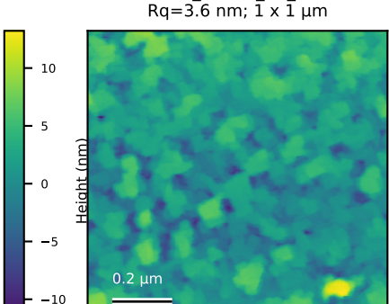
GdSb_N6056_ctr_004 Rq=3.6 nm; 1 x 1 \mu m
