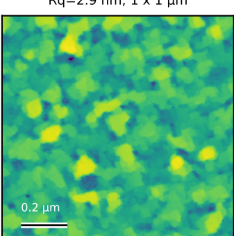
GdSb_N6056_edge_003 Rq=2.9 nm; 1 x 1 \mu m
