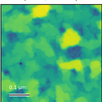
GdSb_N6056_ctr_Copy_001 Rq=3 nm; 0.5 x 0.5 \mu m
