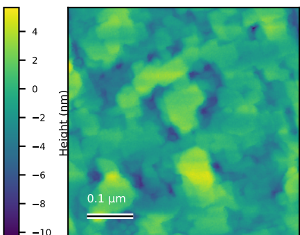
GdSb_N6056_ctr_Copy_000 Rq=2.5 nm; 0.5 x 0.5 \mu m
