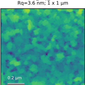
N56_Edg_001 Rq=3.6 nm; 1 x 1 \mu m
