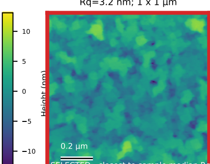
GdSb_N6056_ctr_006 Rq=3.2 nm; 1 x 1 \mu m
