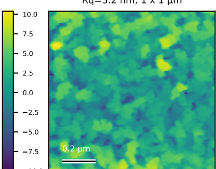
GdSb_N6056_edge_008 Rq=3.2 nm; 1 x 1 \mu m
