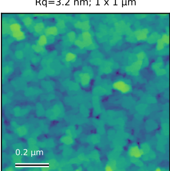
GdSb_N6056_ctr_005 Rq=3.2 nm; 1 x 1 \mu m
