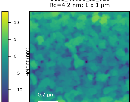
GdSb_N6056_ctr_011 Rq=4.2 nm; 1 x 1 \mu m
