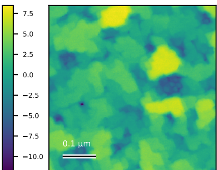
GdSb_N6056_ctr_001 Rq=3 nm; 0.5 x 0.5 \mu m
