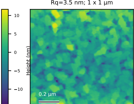
GdSb_N6056_ctr_010 Rq=3.5 nm; 1 x 1 \mu m
