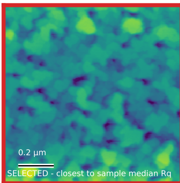
GdSb_N6057_edge_019 Rq=5.3 nm; 1 \times 1 \mu\text{m}
