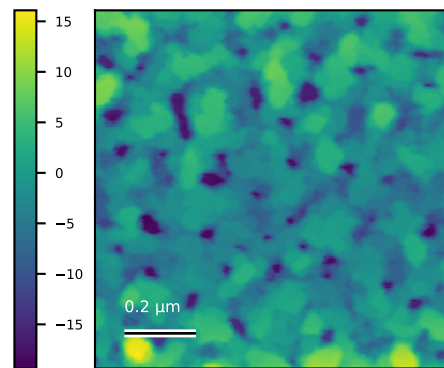
GdSb_N6057_edge_018 Rq=5.5 nm; 1 \times 1 \mu\text{m}
