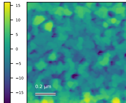
GdSb_N6057_ctr_017 Rq=5.2 nm; 1 \times 1 \mu\text{m}
