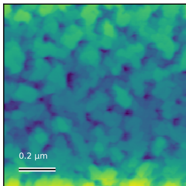
GdSb_N6057_edge_014 Rq=6.5 nm; 1 \times 1 \mu\text{m}
