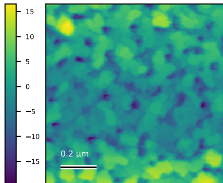
GdSb_N6057_ctr_015 Rq=4.9 nm; 1 \times 1 \mu\text{m}
