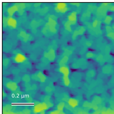
GdSb_N6057_ctr_020 Rq=4.9 nm; 1 \times 1 \mu\text{m}
