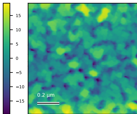
GdSb_N6057_ctr_016 Rq=5.4 nm; 1 \times 1 \mu\text{m}
