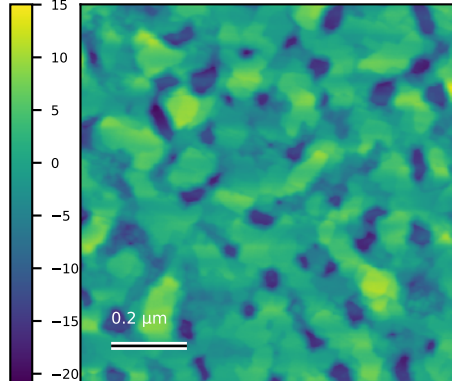
N58_Ctr_003 Rq=5.3 nm; 1 x 1 \mu m
