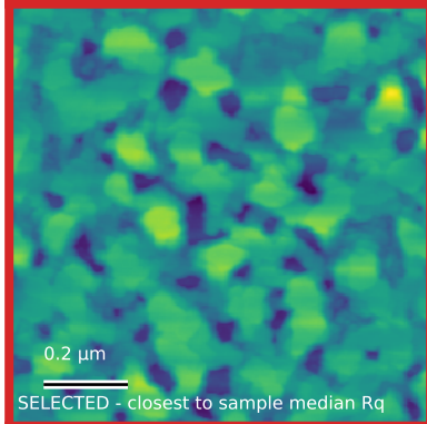
N58_Ctr_000 Rq=5.8 nm; 1 x 1 \mu m
