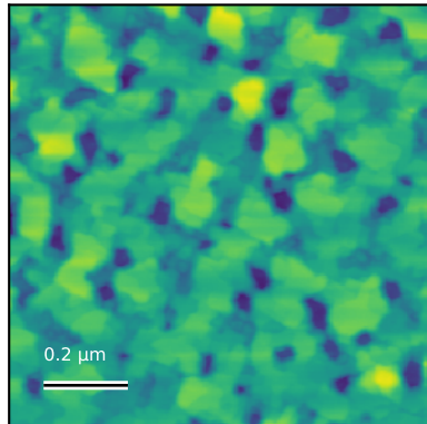
N58_Ctr_002 Rq=5.3 nm; 1 x 1 \mu m
