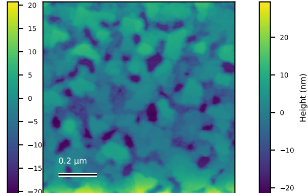
N58_edg_001 Rq=7.5 nm; 1 x 1 \mu m
