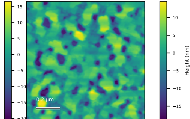
N58_Ctr_001 Rq=5.8 nm; 1 x 1 \mu m
