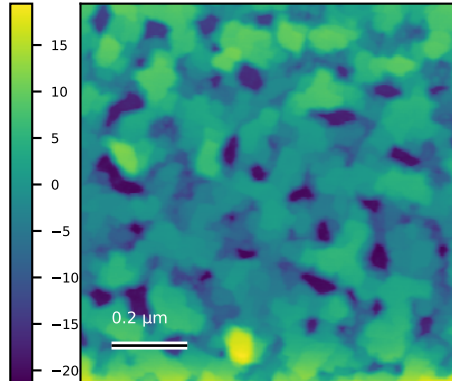
N58_edg_000 Rq=6.8 nm; 1 x 1 \mu m
