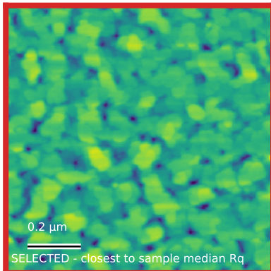
N62_Ctr_001 Rq=3.2 nm; 1 x 1 \mu m
