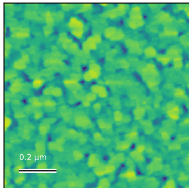
N62_Edg_001 Rq=2.6 nm; 1 x 1 \mu m
