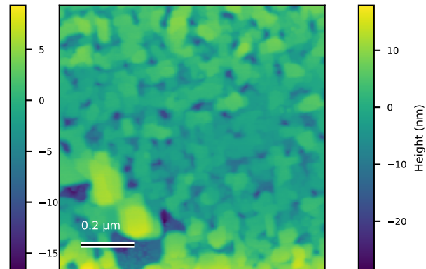
N62_Edg_000 Rq=5.7 nm; 1 x 1 \mu m
