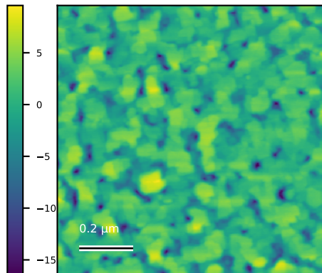
N62_Ctr_002 Rq=3.2 nm; 1 x 1 \mu m
