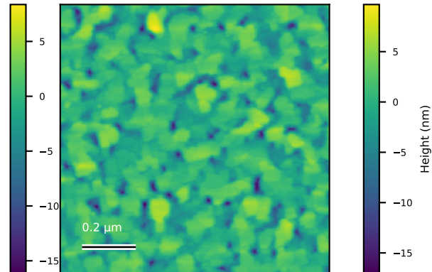
N62_Ctr_003 Rq=3 nm; 1 x 1 \mu m
