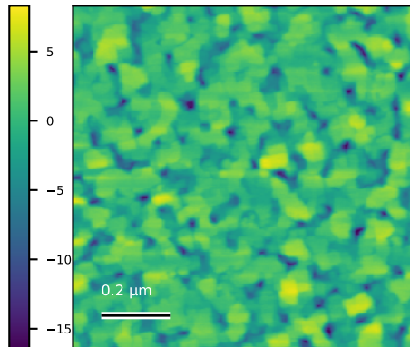
N62_Ctr_000 Rq=2.9 nm; 1 x 1 \mu m
