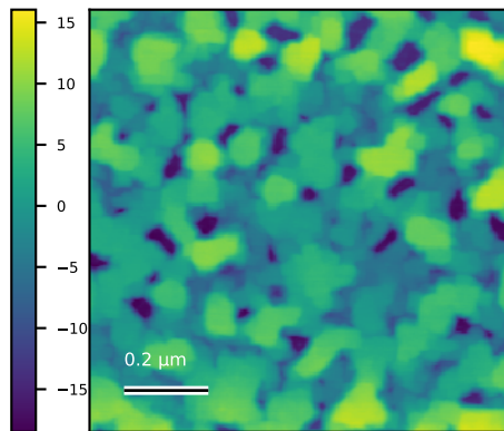
N63_Ctr_002 Rq=6.2 nm; 1 x 1 \mu m
