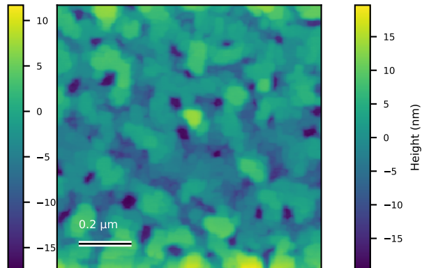
N63_Edg_000 Rq=5.7 nm; 1 x 1 \mu m
