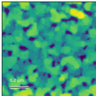
N63_Ctr_003 Rq=5.6 nm; 1 x 1 \mu m
