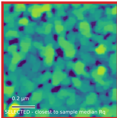
N63_Ctr_001 Rq=6 nm; 1 x 1 \mu m
