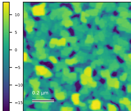
N63_Ctr_004 Rq=5.7 nm; 1 x 1 \mu m
