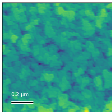
N69_center_200nm_007 Rq=2.7 nm; 1 x 1 \mu\text{m}
