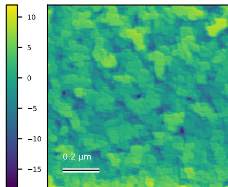
N69_Edg_000 Rq=3.2 nm; 1 x 1 \mu\text{m}
