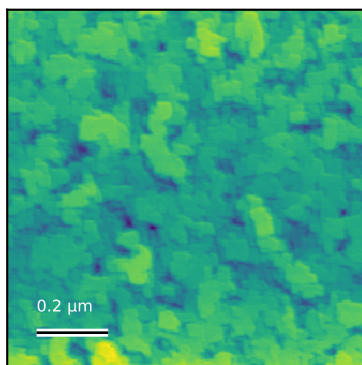
N69_Edg_002 Rq=3.2 nm; 1 x 1 \mu\text{m}
