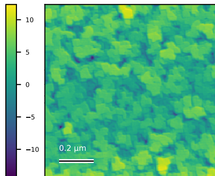
N69_center_200nm_005 Rq=3 nm; 1 x 1 \mu\text{m}
