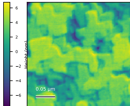
N69_center_200nm_006 Rq=2.1 nm; 0.269531 x 0.269531 \mu\text{m}
