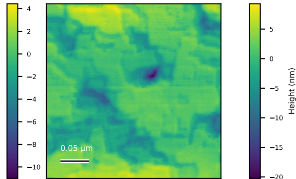
N69_Edg_001 Rq=3.3 nm; 0.304688 x 0.304688 \mu\text{m}
