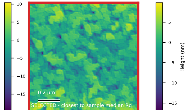
N69_center_003 Rq=3 nm; 1 x 1 \mu\text{m}
