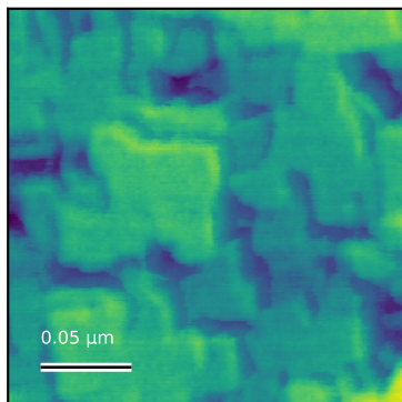
N69_center_200nm_004 Rq=2 nm; 0.21875 x 0.21875 \mu\text{m}
