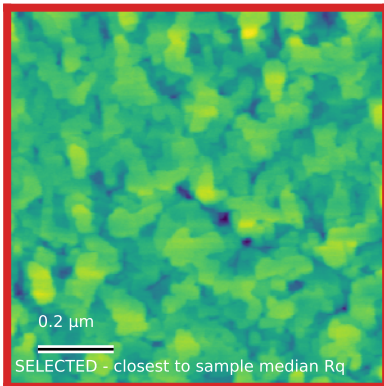
N73_ctr_001 Rq=1.5 nm; 1 x 1 \mu\text{m}
