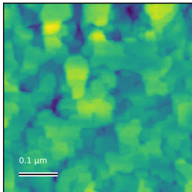
N73_ctr_000 Rq=1.4 nm; 0.488 x 0.488 \mu\text{m}
