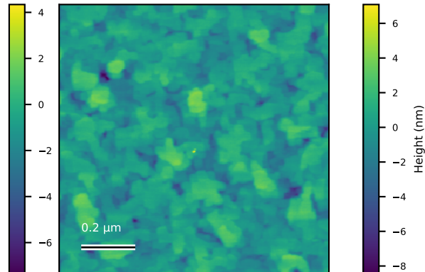
N73_ctr_002 Rq=1.4 nm; 1 x 1 \mu\text{m}
