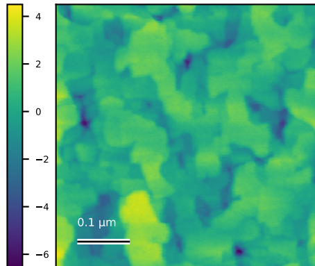
N73_ctr_003 Rq=1.3 nm; 0.5 x 0.5 \mu\text{m}
