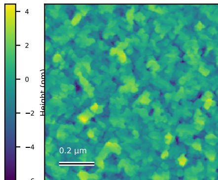
N78_1um_005 Rq=1.3 nm; 1 x 1 \mu\text{m}
