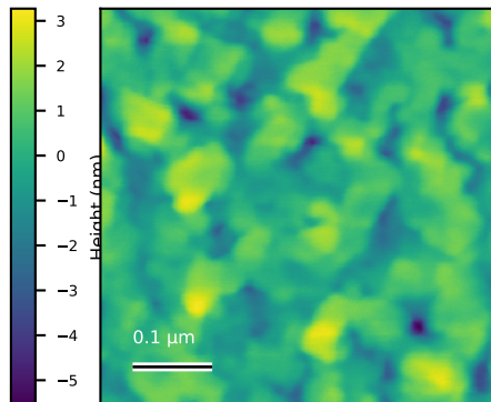
N78_Edg_001 Rq=1.3 nm; 0.5 x 0.5 \mu\text{m}
