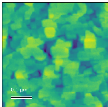
N74_ctr_005 Rq=1.1 nm; 0.5 x 0.5 \mu\text{m}
