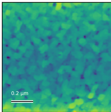
N78_Edg_000 Rq=2.6 nm; 1 x 1 \mu\text{m}
