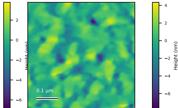
N78_Ctr_001 Rq=1.4 nm; 0.5 x 0.5 \mu\text{m}
