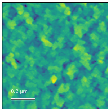
N78_1um_004 Rq=1.2 nm; 0.891 x 0.891 \mu\text{m}
