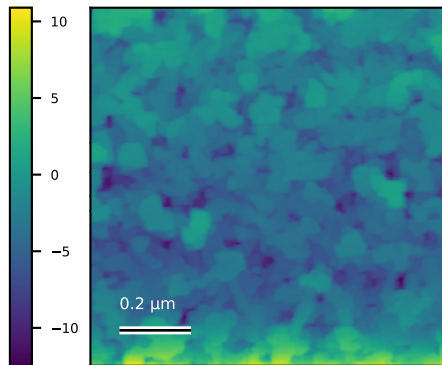
N74_ctr_004 Rq=2.6 nm; 1 x 1 \mu\text{m}
