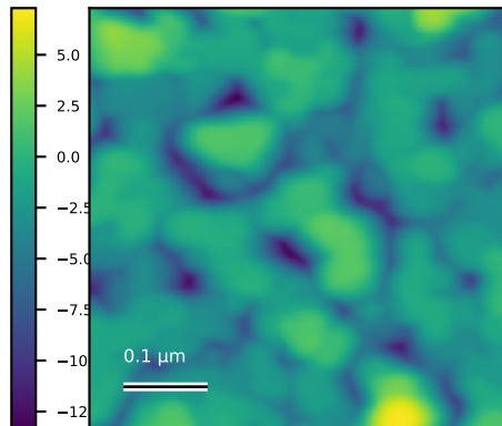
N80_Edg_001 Rq=3.5 nm; 0.5 x 0.5 \mu m
