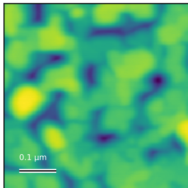
N80_Ctr_001 Rq=3.2 nm; 0.5 x 0.5 \mu m
