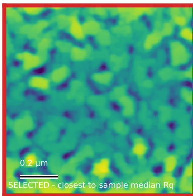
N80_Edg_000 Rq=5.2 nm; 1 x 1 \mu m
