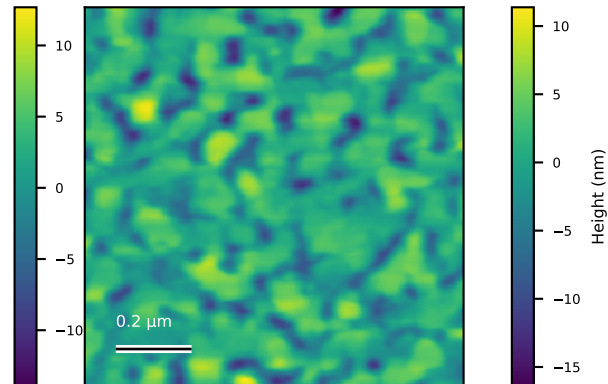
N80_Ctr_000 Rq=3.6 nm; 1 x 1 \mu m
