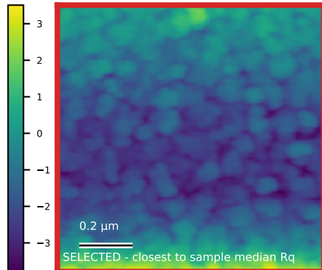
N81_Ctr_000 Rq=3.2 nm; 1 x 1 \mu m
