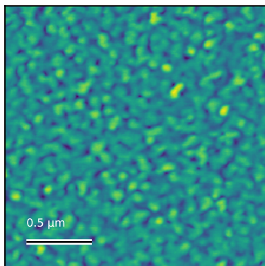
N6081_2um_001 Rq=0.97 nm; 2 x 2 \mu m
