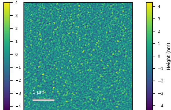
N6081_2um_003 Rq=1 nm; 5 x 5 \mu m
