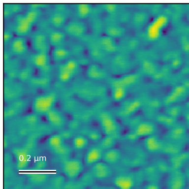
N6081_1um_000 Rq=0.94 nm; 1 x 1 \mu m
