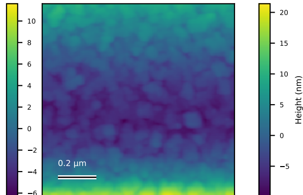
N81_Edg_000 Rq=5.8 nm; 1 x 1 \mu m
