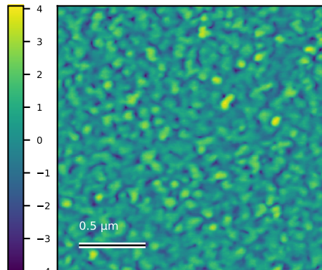
N6081_2um_002 Rq=0.98 nm; 2 x 2 \mu m
