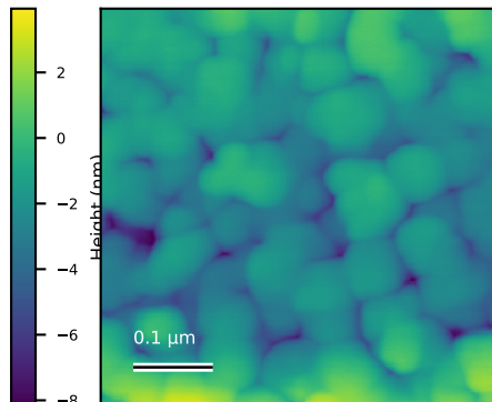
N6084_500_nm_003 Rq=2.2 nm; 0.5 x 0.5 \mu\text{m}
