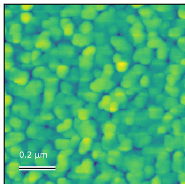
N6084_1um_004 Rq=1.4 nm; 1 x 1 \mu\text{m}
