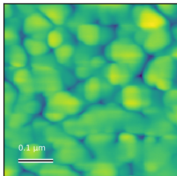
N6084_500_nm_002 Rq=1.3 nm; 0.5 x 0.5 \mu\text{m}
