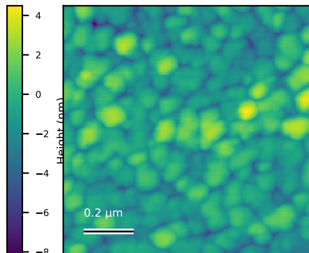
N6084_1um_006 Rq=1.6 nm; 1 x 1 \mu\text{m}
