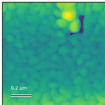
N6084_1um_000 Rq=4.6 nm; 1 x 1 \mu\text{m}
