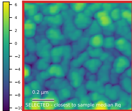
N6085_1um_002 Rq=3.1 nm; 1 × 1 μm
