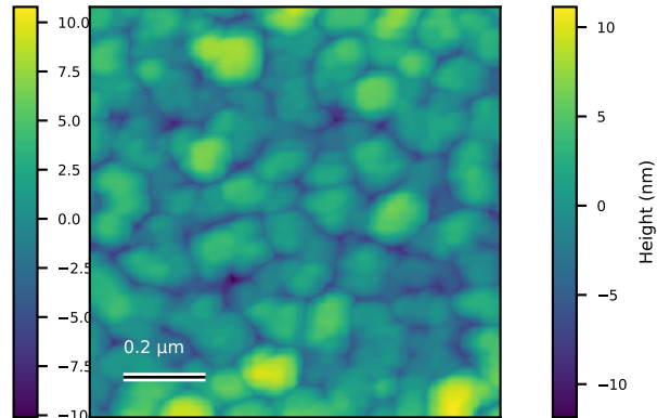
N6085_1um_003 Rq=3.2 nm; 1 × 1 μm
