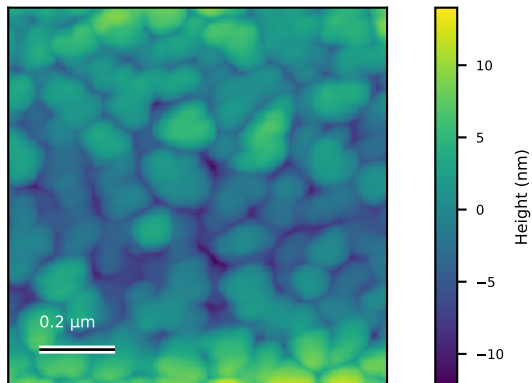
N6085_1um_000 Rq=3.8 nm; 1 × 1 μm
