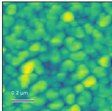
N6085_1um_001 Rq=2.1 nm; 1 × 1 μm
