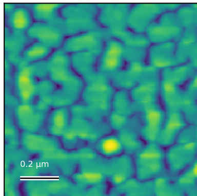
N6093_1um_003 Rq=5.4 nm; 1 x 1 \mu m
