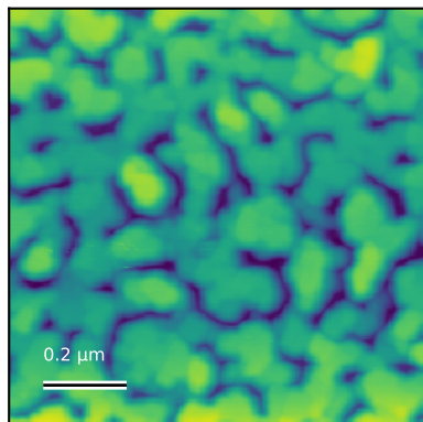
N6093_1um_000 Rq=7.5 nm; 1 x 1 \mu m
