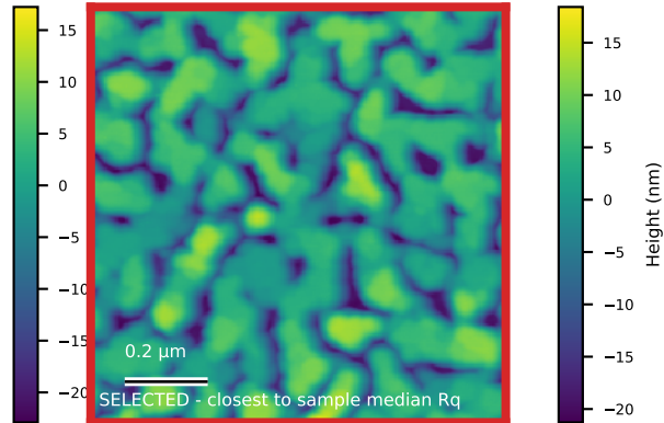
N6093_1um_001 Rq=7.1 nm; 1 x 1 \mu m
