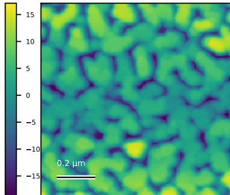
N6093_1um_002 Rq=7 nm; 1 x 1 \mu m
