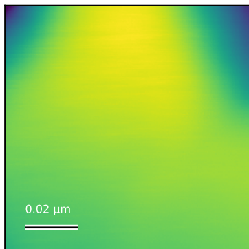
N6095_1um_004 Rq=3.9 nm; 0.09375 x 0.09375 \mu\text{m}
