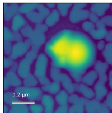
N6095_1um_005 Rq=20 nm; 1 x 1 \mu\text{m}
