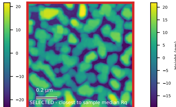
N6095_100_nm_001 Rq=9.9 nm; 1 x 1 \mu\text{m}
