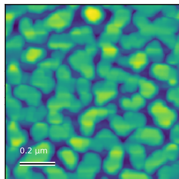
N6095_1um Rq=8.6 nm; 1 x 1 \mu\text{m}
