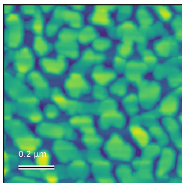
N6095_1um_003 Rq=8.1 nm; 1 x 1 \mu\text{m}
