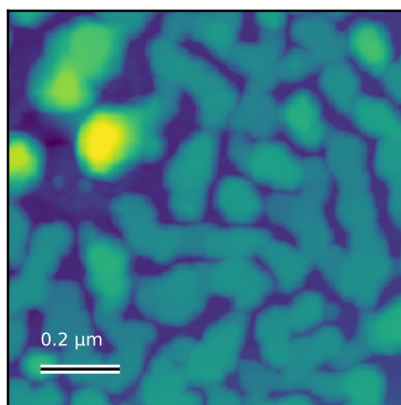
N6095_1um_006 Rq=12 nm; 1 x 1 \mu\text{m}
