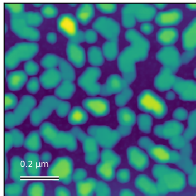
N6099_1um_001 Rq=10 nm; 1 x 1 \mu m
