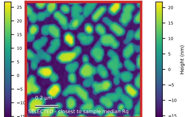
N6099_1um_003 Rq=10 nm; 1 x 1 \mu m
