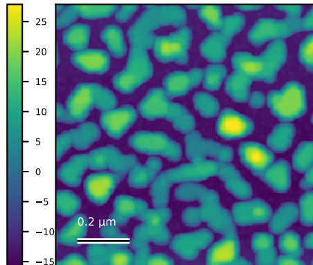
N6099_1um_000 Rq=10 nm; 1 x 1 \mu m
