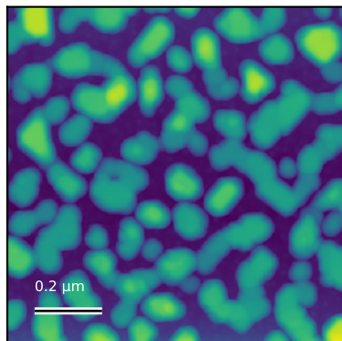
N6099_1um_004 Rq=10 nm; 1 x 1 \mu m
