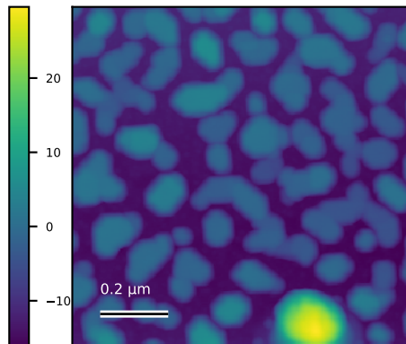
N6099_1um_002 Rq=14 nm; 1 x 1 \mu m
