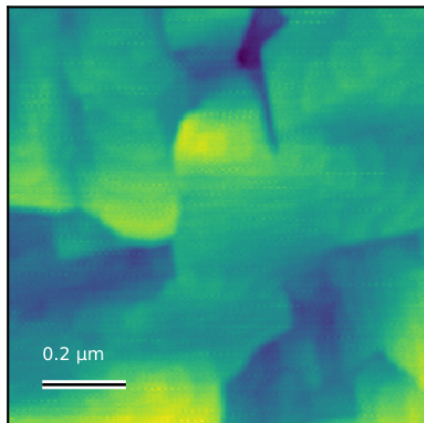
N6101_5um_001 Rq=0.71 nm; 1 x 1 \mu m
