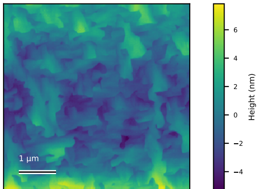
N6101_5um_000 Rq=2.1 nm; 5 x 5 \mu m
