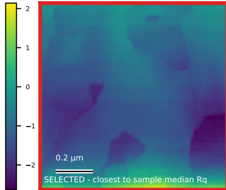
N6101_1um_002 Rq=2.1 nm; 1 x 1 \mu m
