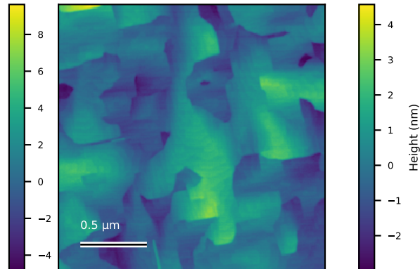
N6101_1um_003 Rq=1.1 nm; 2 x 2 \mu m
