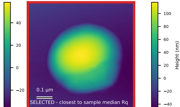
N6102_2um_000 Rq=48 nm; 0.664063 x 0.664063 \mu\text{m}
