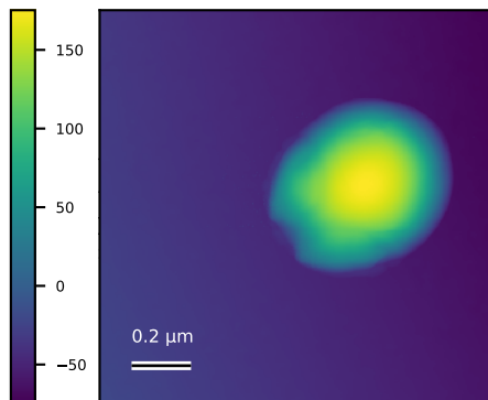
N6102_2um_002 Rq=44 nm; 1.32813 x 1.32813 \mu\text{m}
