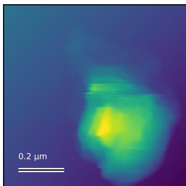
N6102_2um_004 Rq=47 nm; 0.800781 x 0.800781 \mu\text{m}
