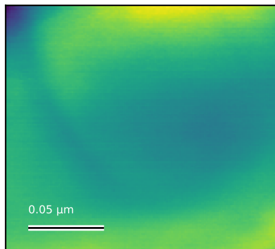
N6102_2um_cs_000 Rq=2.1 nm; 0.178559 x 0.178559 \mu\text{m}
