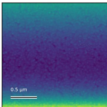
N6102_2um_001 Rq=2.5 nm; 2 x 2 \mu\text{m}
