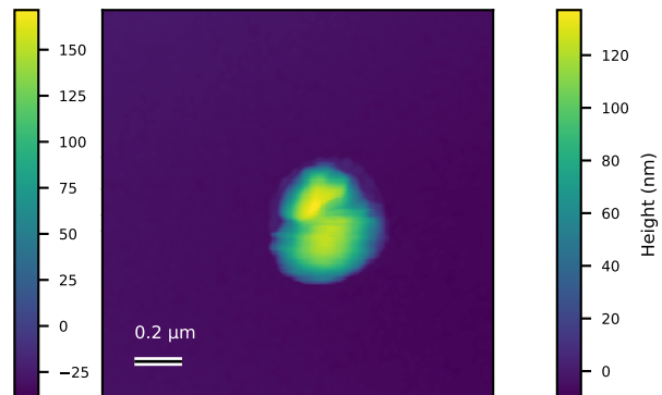
N6102_2um_005 Rq=23 nm; 1.64063 x 1.64063 \mu\text{m}
