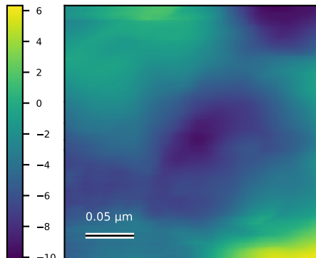
N6102_2um_006 Rq=16 nm; 0.262756 x 0.262756 \mu\text{m}
