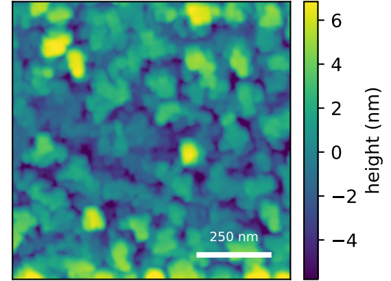
measured AFM Rq=4.09 nm, FSMI=3.62 nm
