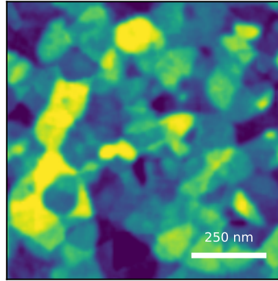
generated AFM Rq=4.07 nm, FSMI=3.42 nm, C=81/100
