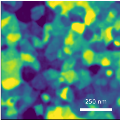
generated AFM Rq=3.13 nm, FSMI=2.60 nm, C=69/100
