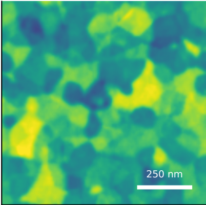
generated AFM Rq=5.17 nm, FSMI=4.33 nm, C=38/100
