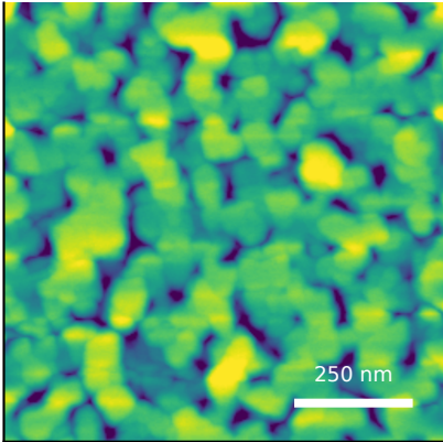
measured AFM Rq=3.09 nm, FSMI=2.92 nm
