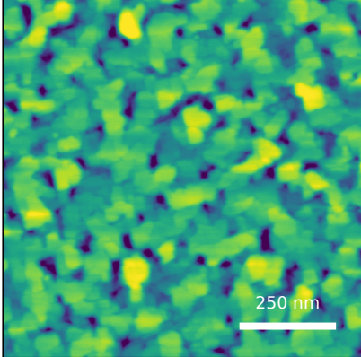
measured AFM Rq=3.13 nm, FSMI=2.46 nm
