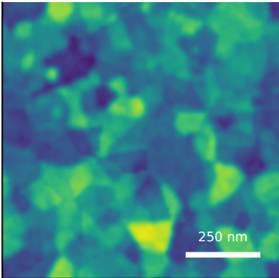
generated AFM Rq=2.61 nm, FSMI=2.23 nm, C=67/100
