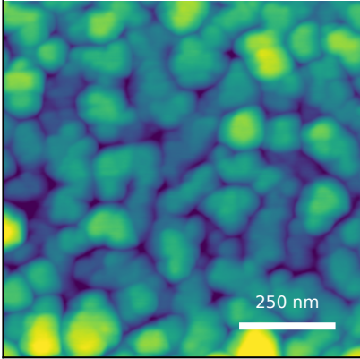
measured AFM Rq=3.18 nm, FSMI=2.06 nm
