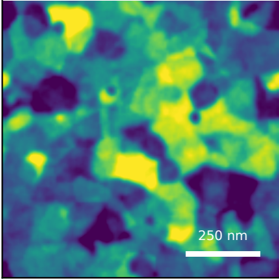
generated AFM Rq=3.97 nm, FSMI=3.31 nm, C=40/100
