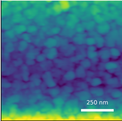
measured AFM Rq=3.23 nm, FSMI=2.66 nm
