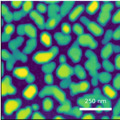
measured AFM Rq=10.32 nm, FSMI=9.32 nm
