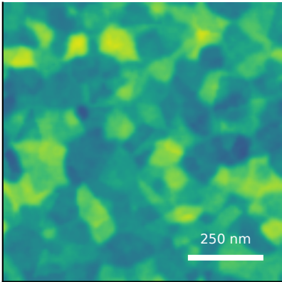
generated AFM Rq=7.25 nm, FSMI=6.44 nm, C=61/100
