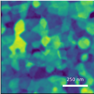
generated AFM Rq=6.96 nm, FSMI=5.22 nm, C=39/100
