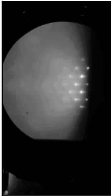
6095 RHEED key frame
