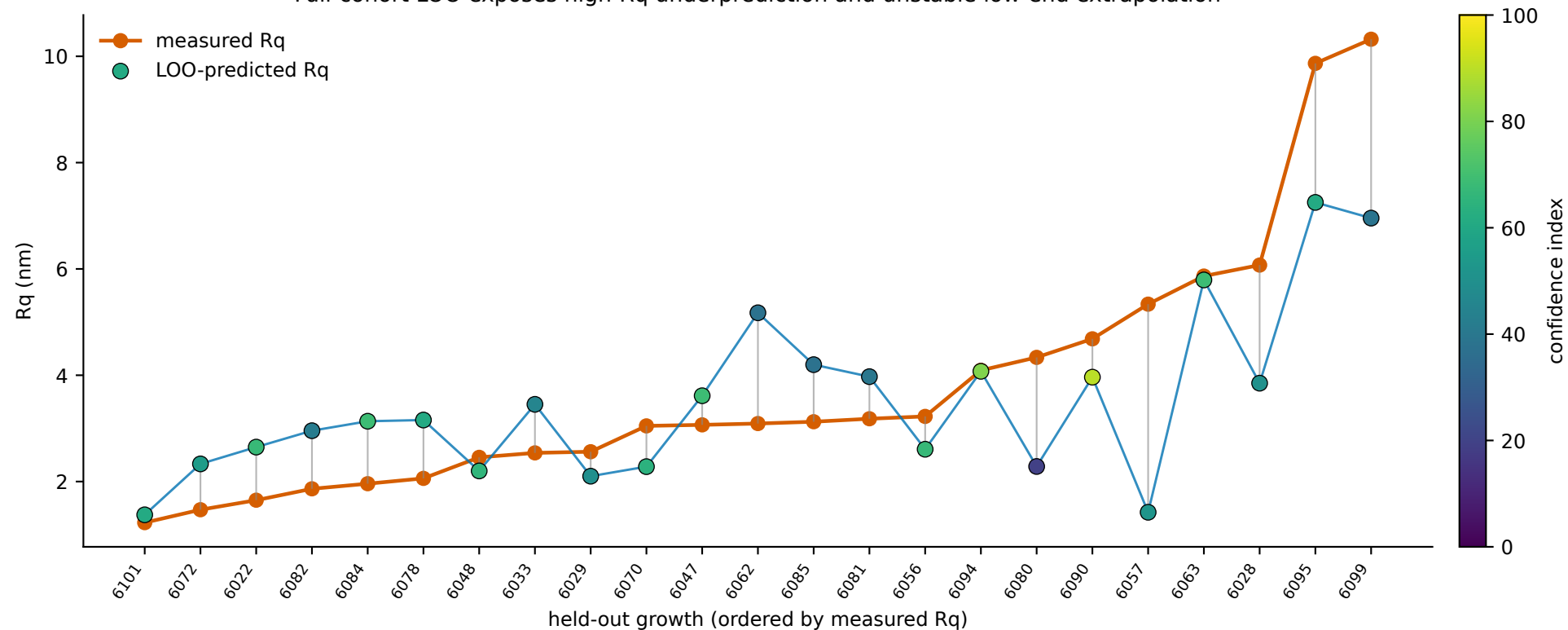
Full-cohort LOO exposes high-Rq underprediction and unstable low-end extrapolation
