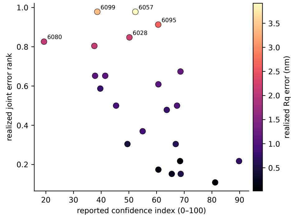
Confidence is error-related: Spearman \rho=-0.65 , p=0.001
