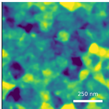
M10 baseline predicted Rq=5.17 nm
