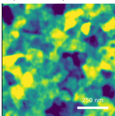
M10 baseline predicted Rq=2.28 nm
