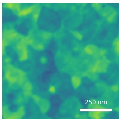
M10 baseline predicted Rq=6.96 nm
