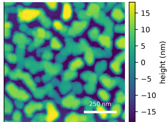
measured AFM Rq=6.07 nm, FSMI=4.94 nm
