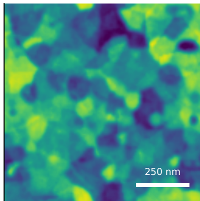
generated AFM Rq=3.85 nm, FSMI=3.43 nm, C=50/100
