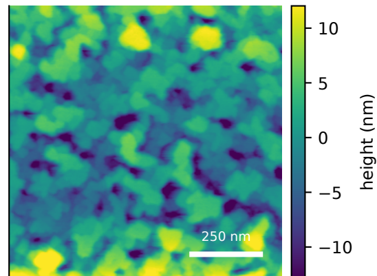
measured AFM Rq=10.32 nm, FSMI=9.32 nm
