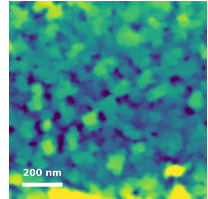
Measured AFM Rq=3.23 nm; shared z=[-7.7, 8.1] nm
