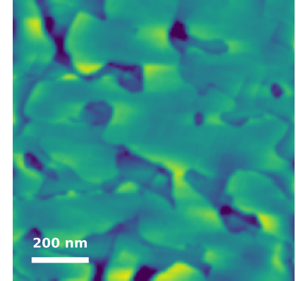
Measured AFM Rq=1.65 nm; shared z=[-5.7, 5.7] nm
