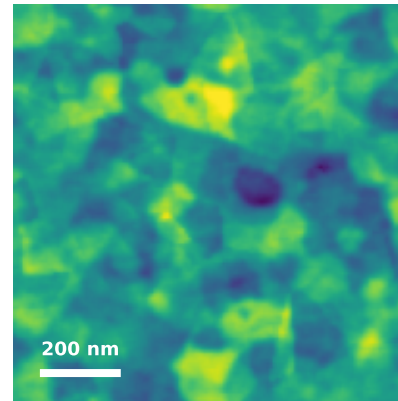
M10 dense islands Rq=2.50 nm
