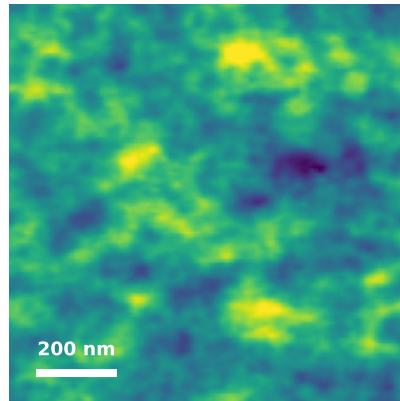
M5 cloud field Rq=2.50 nm
