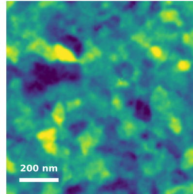
M10 dense islands Rq=3.06 nm
