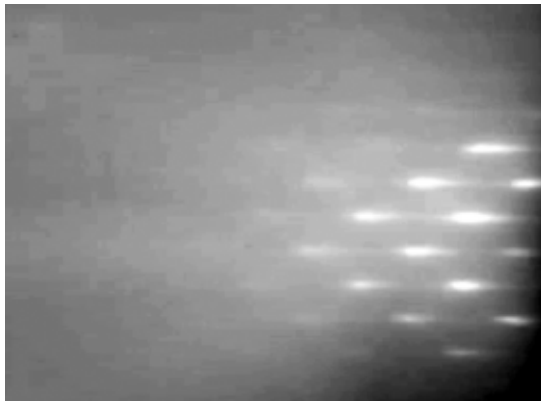
RHEED 6080 condition conf 17/100; morphology conf 69/100 expected island error 1.52z
