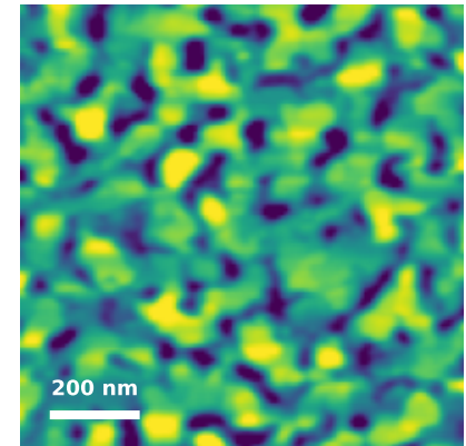
Measured AFM Rq=4.40 nm; shared z=[-9.5, 7.6] nm
