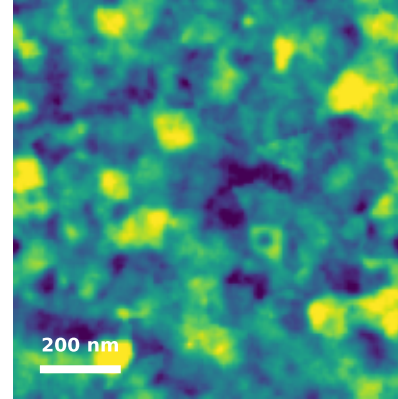
M10 dense islands Rq=2.48 nm
