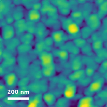
Measured AFM Rq=2.01 nm; shared z=[-5.4, 6.6] nm
