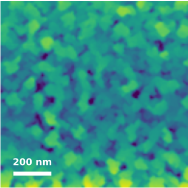
Measured AFM Rq=1.65 nm; shared z=[-5.3, 5.7] nm
