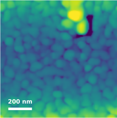
Measured AFM Rq=2.11 nm; shared z=[-5.3, 6.5] nm
