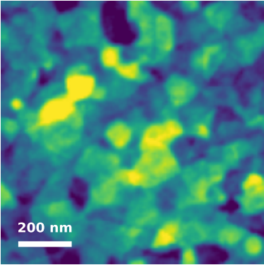
M10 generated Rq=2.84 nm
