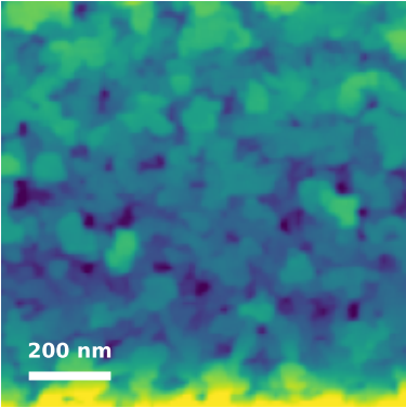
Measured AFM Rq=2.55 nm; shared z=[-6.1, 6.2] nm
