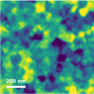
M10 generated Rq=2.48 nm
