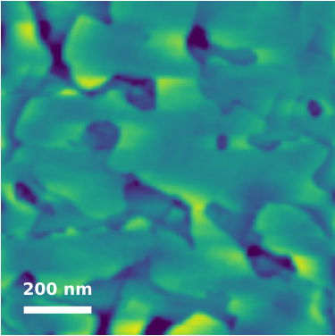
Measured AFM Rq=1.86 nm; shared z=[-5.1, 6.0] nm
