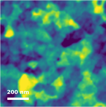
M10 generated Rq=2.66 nm
