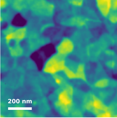
M10 generated Rq=2.54 nm
