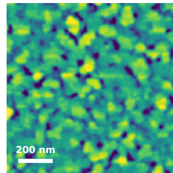
Measured AFM Rq=3.09 nm
