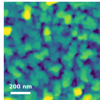
Measured AFM Rq=2.56 nm
