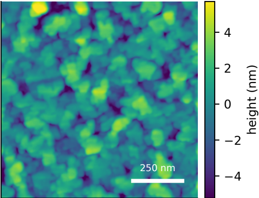
measured AFM Rq=2.54 nm, FSMI=2.13 nm
