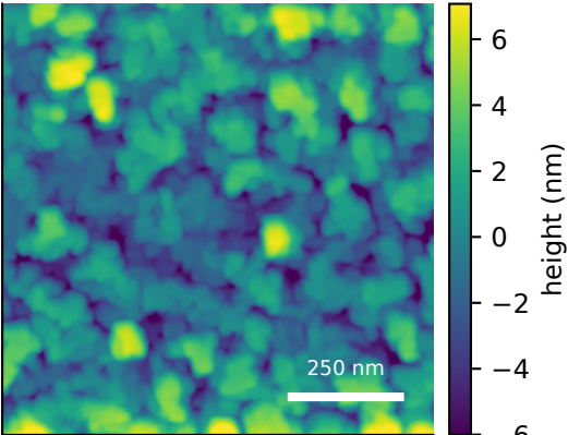
measured AFM Rq=2.56 nm, FSMI=2.22 nm
