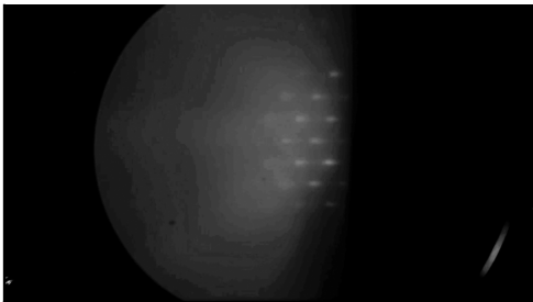
6070 RHEED key frame
