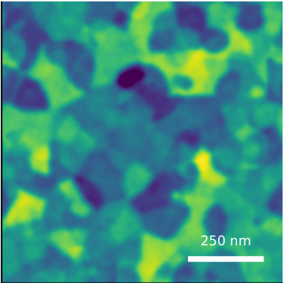
generated AFM Rq=2.89 nm, FSMI=2.95 nm, C=94/100
