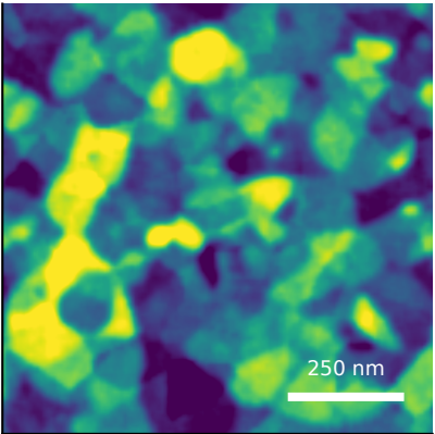
generated AFM Rq=2.21 nm, FSMI=1.63 nm, C=100/100
