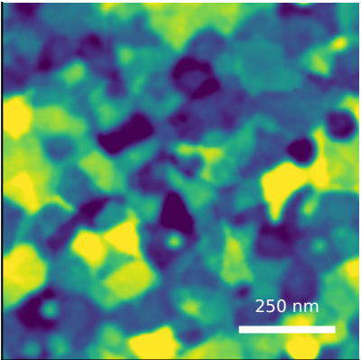
generated AFM Rq=3.67 nm, FSMI=2.69 nm, C=86/100
