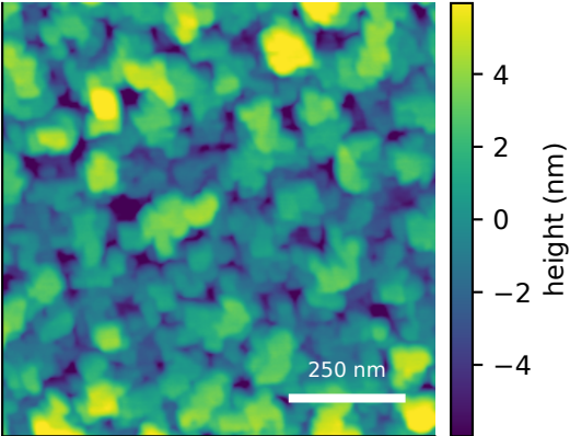
measured AFM Rq=3.05 nm, FSMI=2.62 nm
