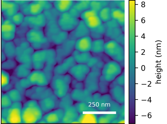
measured AFM Rq=3.18 nm, FSMI=2.06 nm
