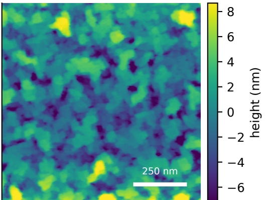
measured AFM Rq=3.23 nm, FSMI=2.66 nm
