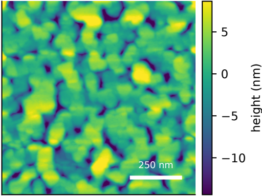
measured AFM Rq=3.09 nm, FSMI=2.92 nm
