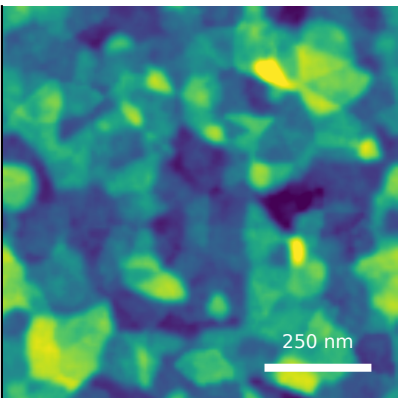
generated AFM Rq=3.28 nm, FSMI=3.39 nm, C=79/100
