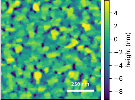
measured AFM Rq=3.13 nm, FSMI=2.46 nm
