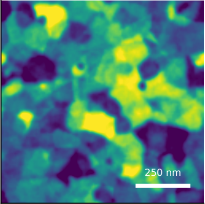
generated AFM Rq=4.13 nm, FSMI=3.72 nm, C=63/100
