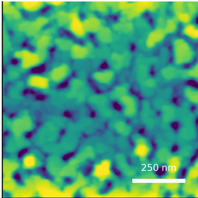
measured AFM Rq=4.69 nm, FSMI=3.17 nm
