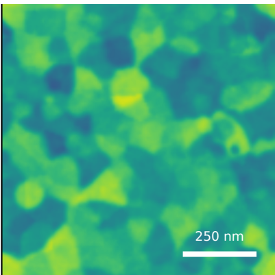
generated AFM Rq=3.37 nm, FSMI=1.88 nm, C=94/100
