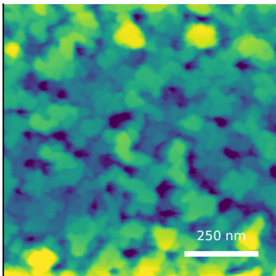
measured AFM Rq=5.87 nm, FSMI=4.88 nm
