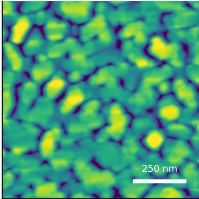
measured AFM Rq=4.34 nm, FSMI=3.81 nm
