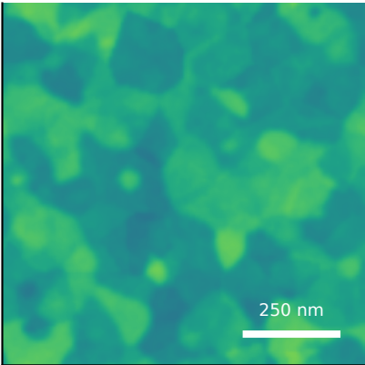
generated AFM Rq=2.94 nm, FSMI=2.06 nm, C=100/100
