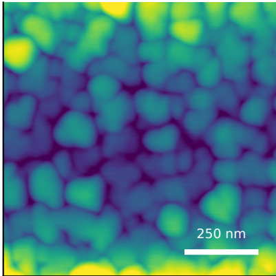
measured AFM Rq=5.34 nm, FSMI=4.21 nm
