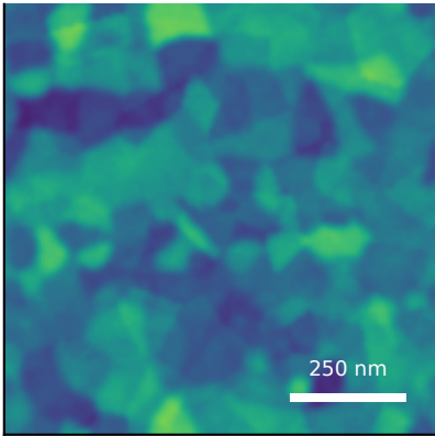
generated AFM Rq=4.45 nm, FSMI=2.78 nm, C=35/100
