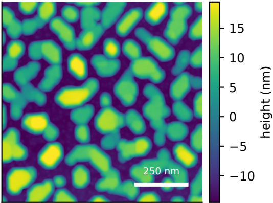
measured AFM Rq=10.32 nm, FSMI=9.32 nm
