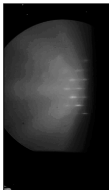
6101 RHEED measured Rq=1.23 nm
