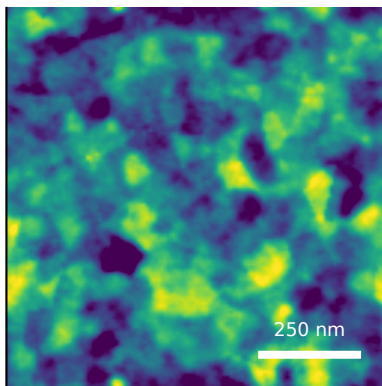
M10 baseline predicted Rq=3.16 nm
