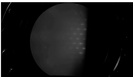
6080 RHEED measured Rq=4.34 nm
