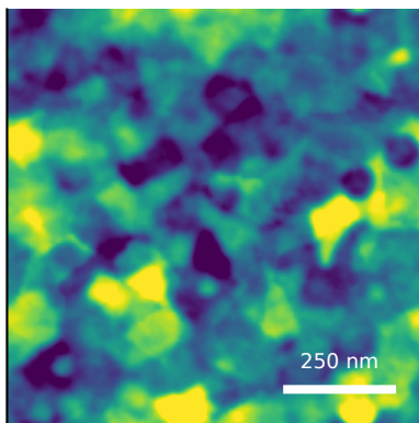
M10 baseline predicted Rq=3.44 nm
