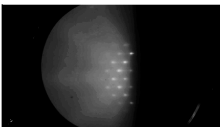
6062 RHEED measured Rq=3.09 nm
