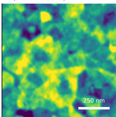
M10 baseline predicted Rq=1.88 nm
