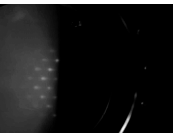
6063 RHEED key frame
