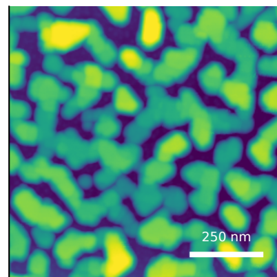
measured AFM Rq=5.34 nm, FSML=4.21 nm
