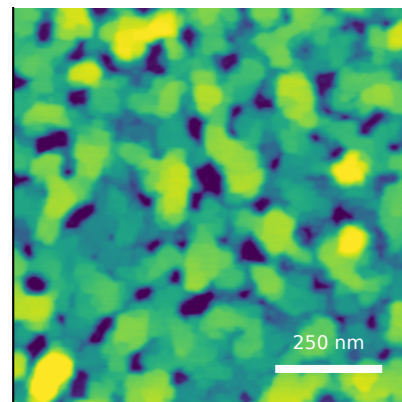
measured AFM Rq=5.87 nm, FSML=4.88 nm
