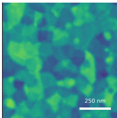
generated AFM Rq=2.64 nm, FSML=2.90 nm, C=92/100
