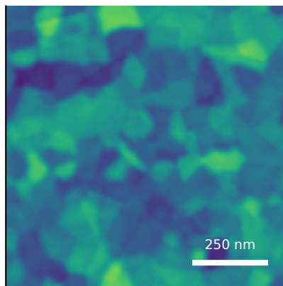
generated AFM Rq=4.51 nm, FSML=2.58 nm, C=65/100
