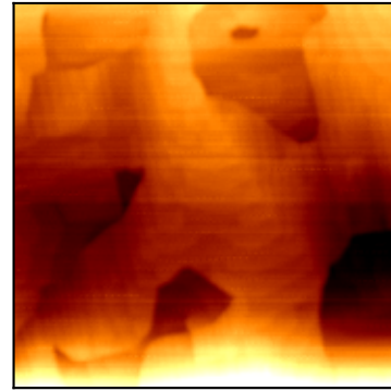
measured AFM Rq=1.47
