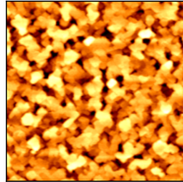
measured AFM Rq=1.65
