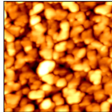
measured AFM Rq=2.01
