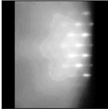
auto RHEED | Cq=73
